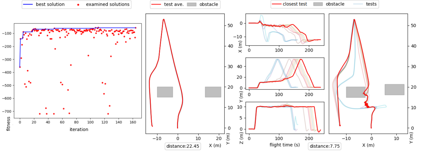
Fig. 2: RQ 1 Fitness progress over iterations (left), RQ 2 Seed (middle) and Final solutions (right)
