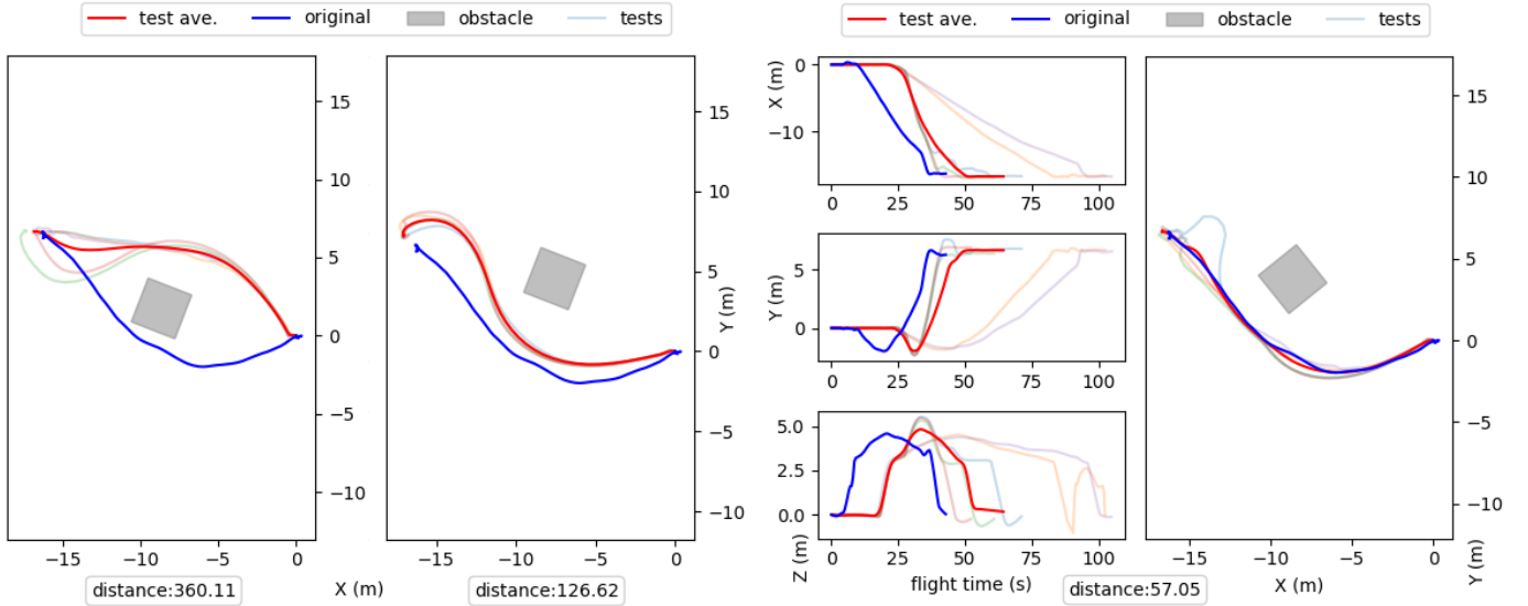
Fig. 1: RQ 1 Seeds 1 and 2 (left) and Final (right) solutions (simulated in Gazebo) compared to the real-world flight
